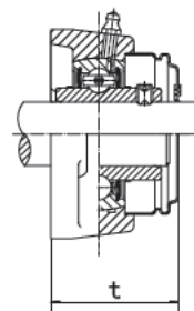
UCFL-C1(D1)
