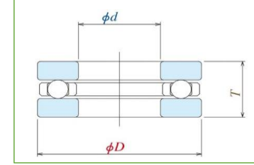
FLAT WASHER TYPE
