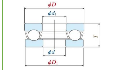
F-G SERIES GROOVED WASHER TYPE
